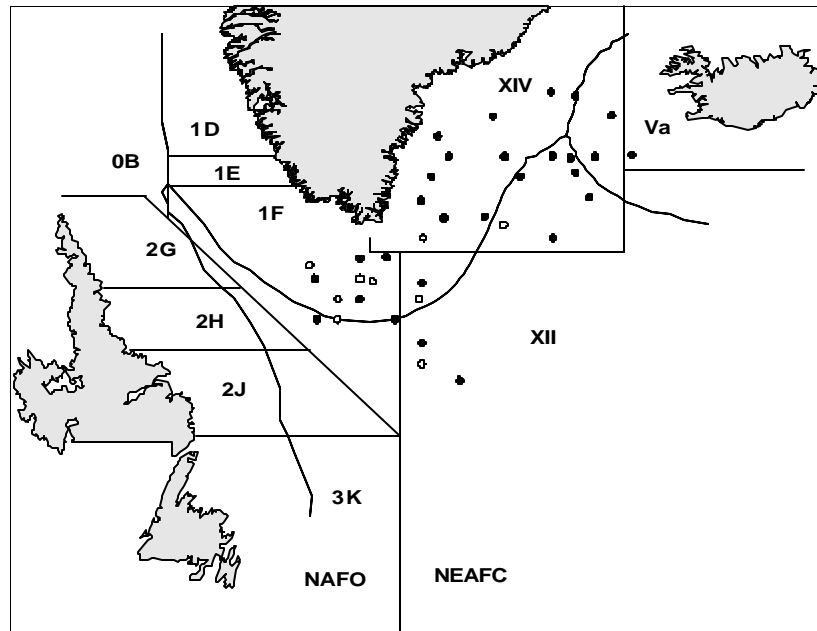
Fig. 1: Stations where otolith samples of pelagic S. mentella were collected in the Irminger Sea in June/July 1999 (Open circles: station shallower than 500 m; filled circles: station deeper than 500 m).
