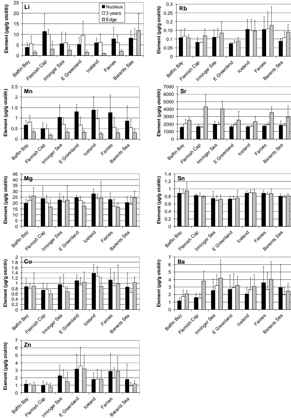
Fig. 3. Mean concentrations (+ standard deviation) of 9 elements determined in S. mentella otoliths from 7 different regions in the North Atlantic.
