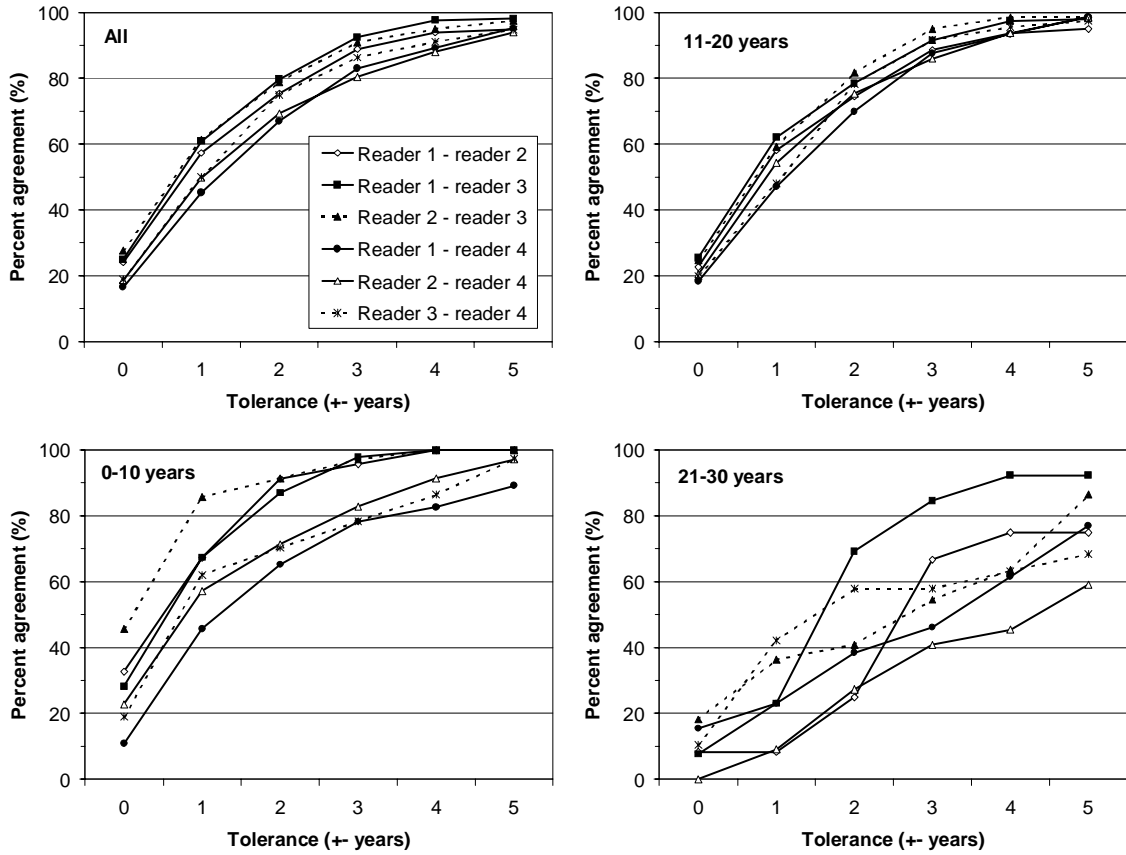
Fig. 2. Percent agreement plots for the reader comparisons based on the S. marinus otoliths from the Icelandic shelf (see Stransky et al. 2001, adding readings of Partner 2 carried out in 2002, Stransky et al. 2002) for a tolerance level (deviation of assigned ages between both readers) of \pm 0 (total agreement) to \pm 5 years. These were applied to all age groups and sub-sets of age ranges assigned by the first reader.
